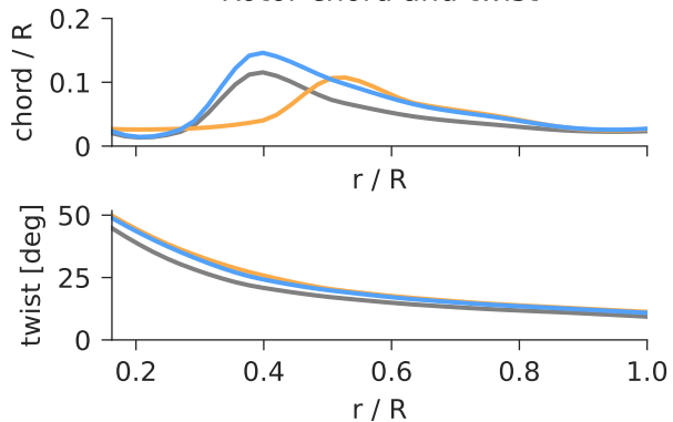
Rotor chord and twist
