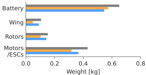
Component weight
